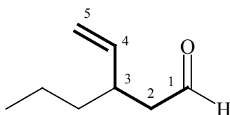
3-Propilpent-4-enal
