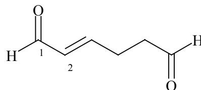
trans -Hex-2-enodial
