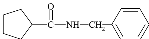
N -Bencilciclopentanocarboxamida
