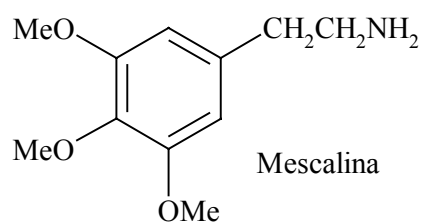
Mescalina 3,4,5-Trimetoxifeniletilamina
