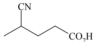
4-Cianopentanoico
