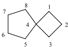
espiro[3,4]octano
