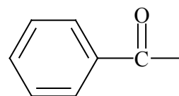
Benzoilo
