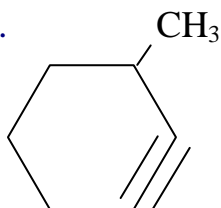
3-metilciclohexino 3-methylcyclohexyne
