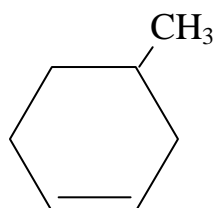
4-metilciclohexeno 4-methylcyclohexene
